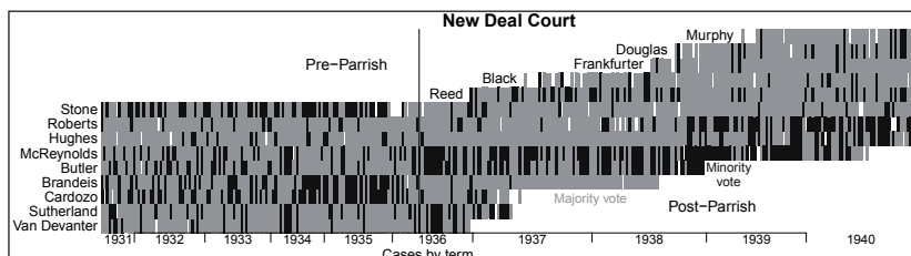
Figure 1. Votes in all nonunanimous cases for the 1931–1940 terms. Justices on the y-axis are sorted by years of service and cases are sorted by dates of decision. Gray (black) cells indicate a majority (minority) vote. The vertical line denotes the Parrish case, decided in the 1936 term, with a formal decision issued on March 29, 1937. This figure demonstrates a marked rupture in voting patterns around the time of the case.
