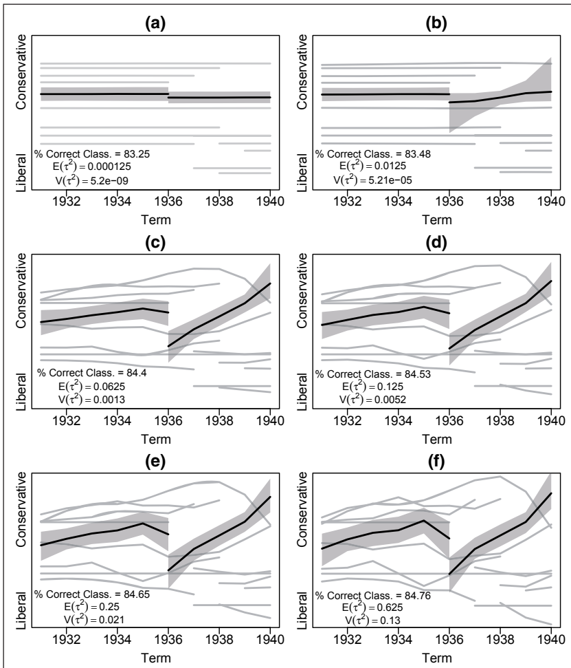
Figure 12. Ideal point estimates for the 1931-1941 period under different prior assumptions for how smoothly views change ( \tau^2 ). In the lower left hand corner of each panel we report the in-sample percentage of correctly classified votes, the prior mean and variance of the smoothness parameter ( \tau^2 ). As the panels progress from (a) to (f) the prior mean and variance increase, meaning that views are allowed to change quickly across time. Results assume that Justices Black, Stone, and Van Devanter are constant. The prior specification depicted in panel (c) is that used in Section 5.2. Evidence of the Roberts shift remains even when views are assumed to be almost constant (i.e., when \tau^2 is forced by prior assumption to take values very close to 0, equivalent to complete pooling of data across time). Roberts's, rightward drift after 1937 remains, to varying degrees, under all prior specifications shown in the figure.
