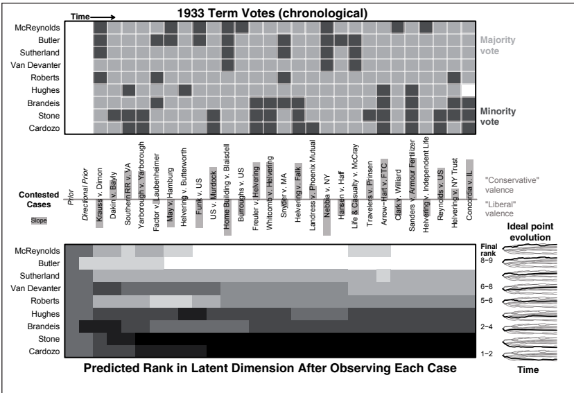
Figure 4. Illustration of “Bayesian learning” about ideal points of justices. This figure illustrates how we update beliefs about the ranks of the justices as nonunanimous cases from the 1933 term are issued chronologically. The top panel presents data on votes cast in each in the order issued. Each column represents one case, and the gray and black cells represent votes by each of the nine justices (in rows) for the majority or minority, respectively. The bottom panel represents the predicted rank of justices at each point in time, where Justice Brandeis is assumed to be on the opposite sides of the median rank from Justice Butler, solely for directional interpretation. The first column of uniform gray represents our “prior” of no differences between the justices, associated with no votes on the top panel. The second column represents a “directional prior,” assuming Brandeis and Butler to be ranked on opposite sides of the median rank. As each case is decided our belief is “updated.” The bars behind the names of cases represent how much weight is given to each case and the estimated direction (i.e., the slope in each case model). Cases with low weight are those that are unconventional according to this ranking (e.g., Factor v. Laubheimer , in which Justices Brandeis, Roberts, and Butler dissented). The bottom right presents the evolution of ideal points of each justice in the latent dimension, contrasted in each instance with the other justices.
