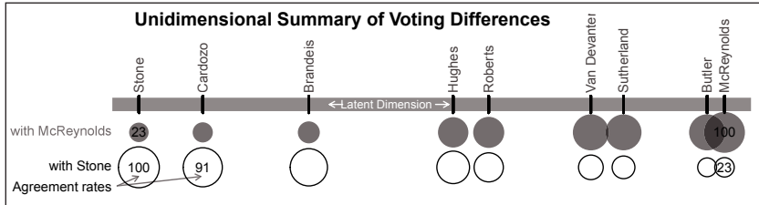
Figure 2. Illustration of location in unidimensional space as a summary of voting differences between justices. The x-axis represents a single latent dimension on which justices might be located, marked by black vertical bars. For example, Justices Stone, Cardozo, and Brandeis are each to the “left” of Chief Justice Hughes. The space between the justices is proportional to how much they agree with each other. The bottom dots plot example pairwise agreement rates between each of the justices and Justices McReynolds and Stone for the Parrish Court, with the area proportional to the agreement rate. Agreements with Justice McReynolds generally increase from left to right, while agreements with Justice Stone generally decrease.
