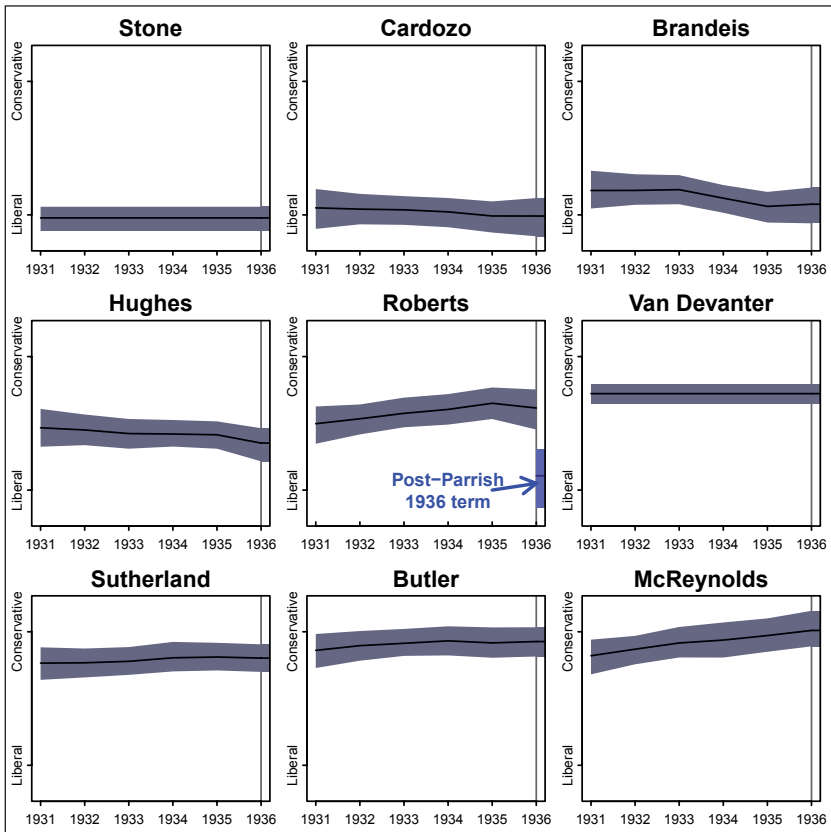
Figure 8. Dynamic ideal point estimates for the Parrish Court. Solid lines are posterior median and the shaded regions are the pointwise 95 percent posterior credible bands. Note the dramatic shift to a more liberal position by Justice Roberts after Parrish .
