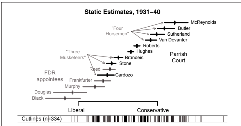
Figure 5. Static (median) ideal point estimates with 95 percent credible intervals for the 1931–1940 terms. Justices are sorted from left to right by median ideal point. Ideal points for justices serving on or before the Parrish term are plotted in black, and others in gray. Bottom strip presents estimated splits between the majority in minority in 334 cases ( \kappa from Appendix A). Static ideal points capture key conventional understandings of the jurisprudence of these justices—i.e., the major cleavages in the Parrish Court between the “Four Horsemen” and the “Three Musketeers”; the center of the Court occupied by Roberts and Hughes; and the liberal turn of the Roosevelt appointees.
