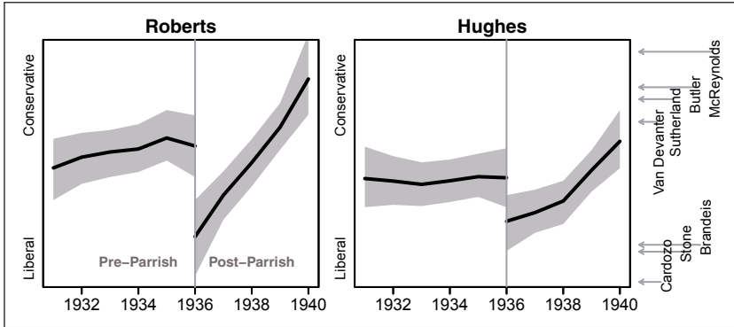
Figure 13. This figure plots dynamic ideal points with separate pre- and post- Parrish trends for Justice Roberts and Chief Justice Hughes. The solid lines represent the pointwise posterior median ideal points and the gray bands provide pointwise 95 percent credible regions. Justice Roberts and, to a lesser extent, Chief Justice Hughes experience sharp shifts to the left in the 1936 term. For reference, arrows on the right provide posterior median ideal points of justices other than Roberts and Hughes on the Court in the 1936 term.
